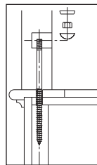
LJ-3008-10 NEWEL POST FASTENER 10-3/4"
