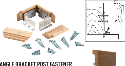
LJ-3009 - 3" Angle Bracket Post Fastener Kit
