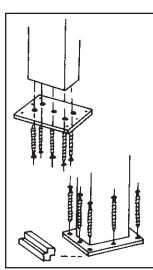
ANGLE BRACKET POST FASTENER
