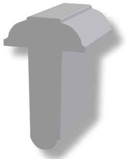
1305 - 1 \frac{3}{8} " Door 1 \frac{1}{8} " x 1 \frac{15}{16} " 8' pieces
